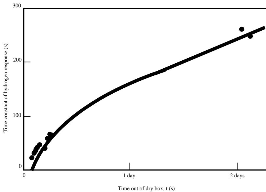
Figure 8. Sensor response time constant for film (17 nm Ag/330 nm WO 3 /100 nm Pd) over a period of 2 days. The sample was exposed to 5% H 2 in air for periods of about 2 minutes, then to dry air. The response time constant was measured away from the SPR, at 800 nm. The fitted curve varies as the square root of time.
