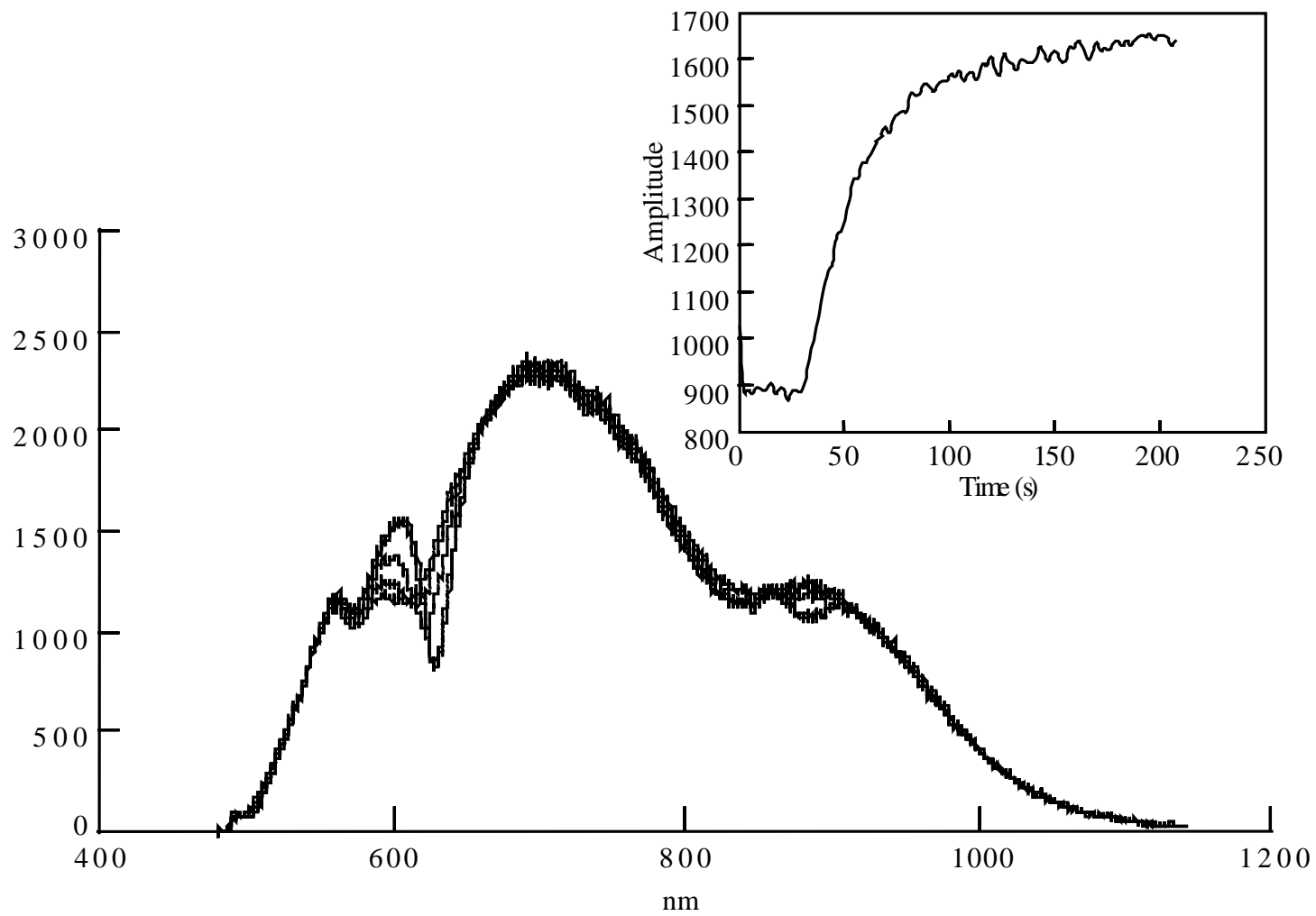
Figure 5. Selected reflectance spectra from a time series during exposure to 5% H 2 in air. The inset shows reflected intensity at 627 nm versus time. The coating is 40 nm Au/600 nm WO 3 /3 nm Pd.
